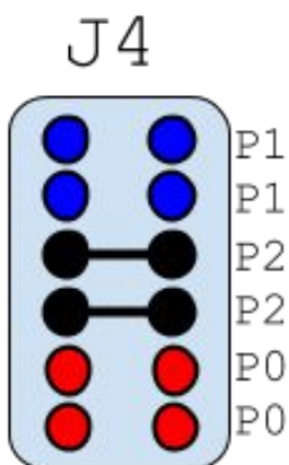
Picture 8. Proper Installation of Jumpers
